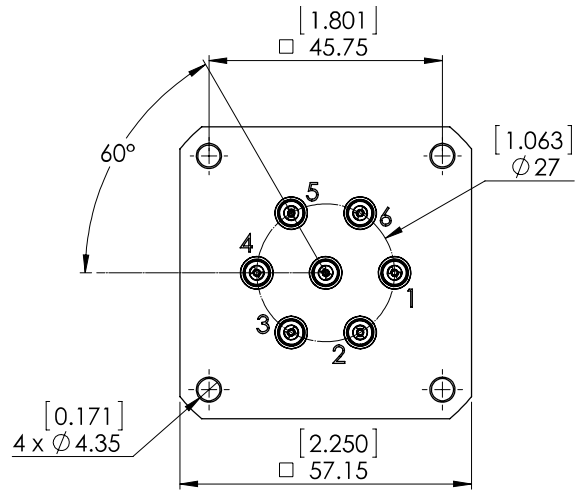
SMA 2.9 Connectors
