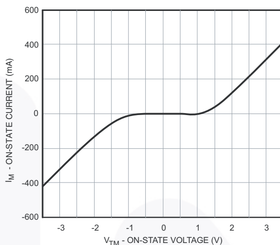
Figure 4. On-State Characteristics
