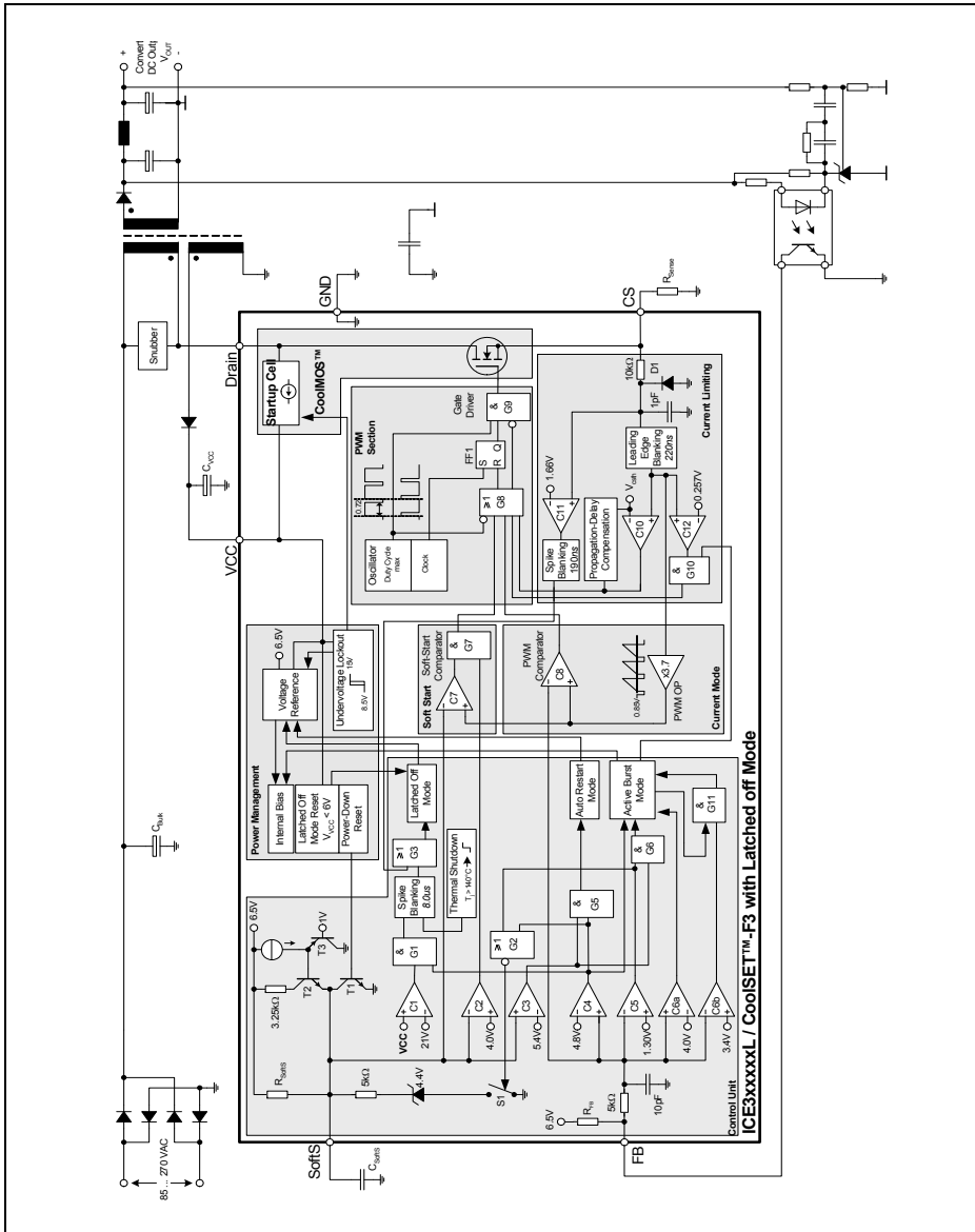
Figure 2 Representative Blockdiagram
