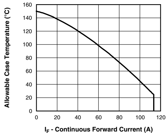
Fig. 7 - Maximum DC Forward Current vs. Case Temperature
