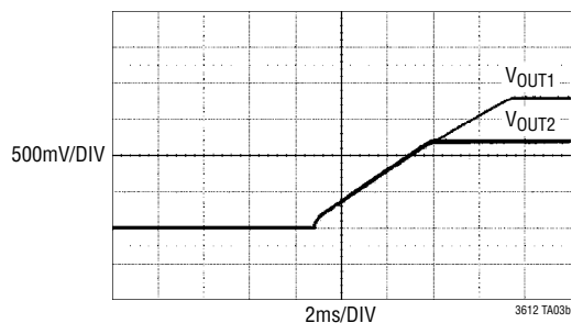
Coincident Start-Up
