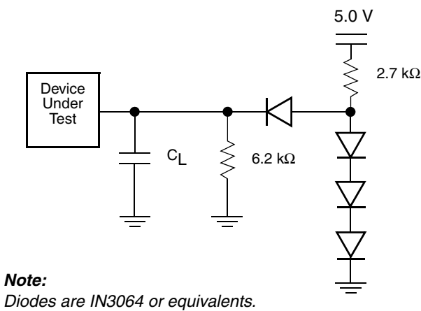
Figure 9. Test Setup
