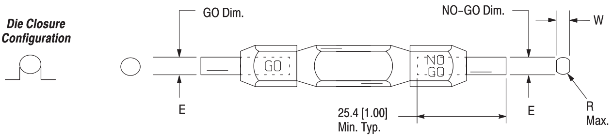
SUGGESTED PLUG GAGE DESIGN FOR INSULATION SEALING CRIMP SECTION
