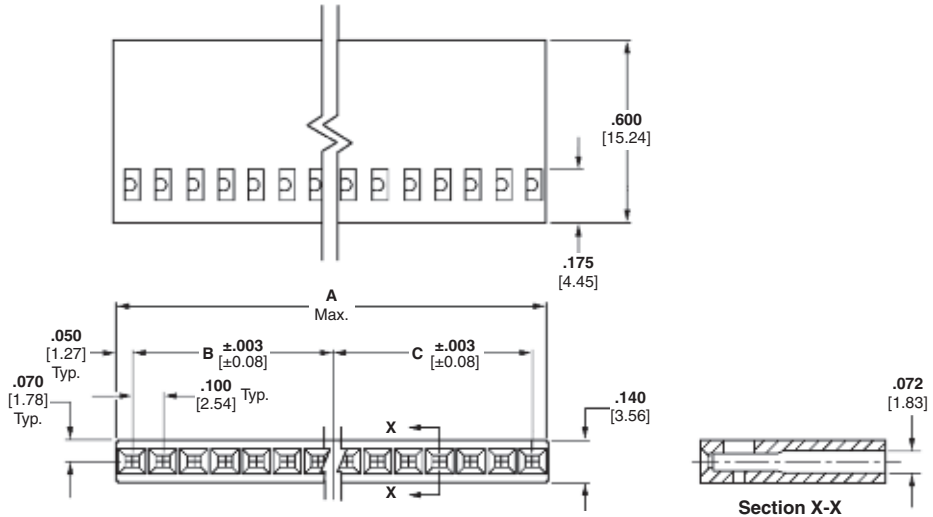
Section X-X
