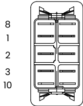
BOTTOM VIEW TERMINAL ARRANGEMENT 10 TERMINAL BASE
