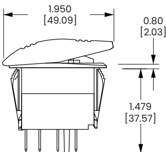
8 TERMINAL BASE W/O BARRIERS
