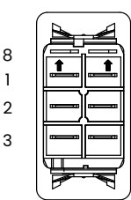
BOTTOM VIEW TERMINAL ARRANGEMENT 8 TERMINAL BASE
