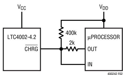
Figure 2. Microprocessor Interface
