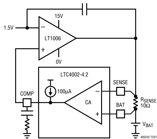
Test Circuit 1
