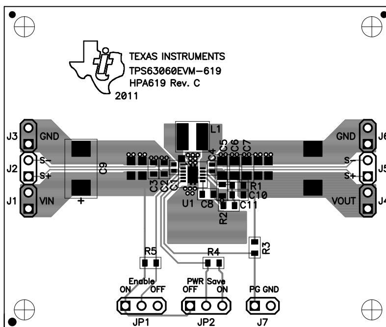
Figure 7. Assembly Layer
