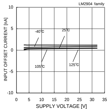
Fig. 66 Input Offset Current – Supply Voltage ( V_{icm}=0[V] , V_{OUT}=1.4[V] )
