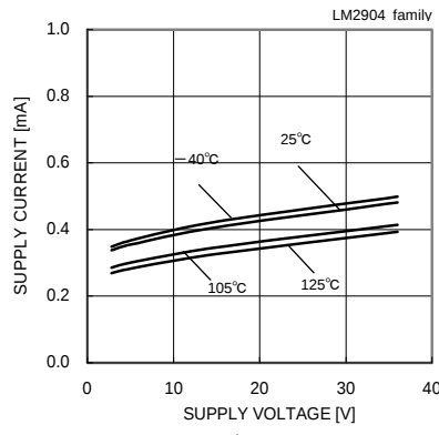
Fig. 50 Supply Current – Supply Voltage
