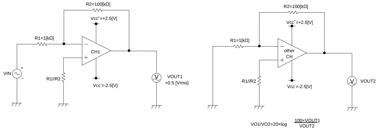
Fig.101 Measurement Circuit3
