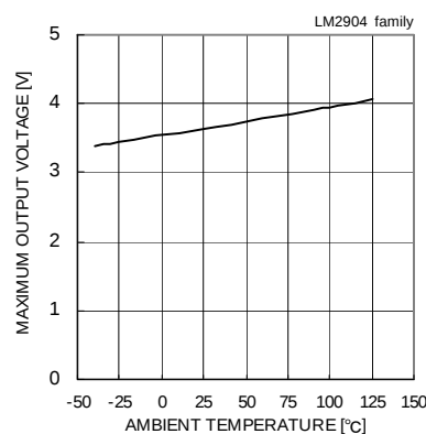
Fig. 53 Maximum Output Voltage – Ambient Temperature ( V_{CC}=5[V] , R_L=2[k\Omega] )
