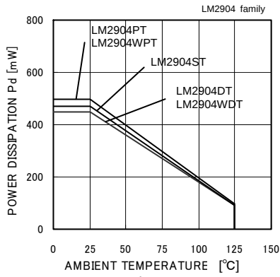
Fig. 49 Derating Curve
