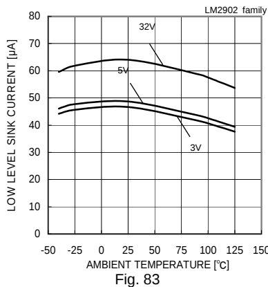
Fig. 83 Low Level Sink Current – Ambient Temperature ( V_{OUT}=0.2[V] )
