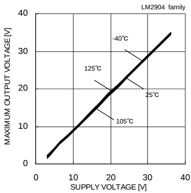
Fig. 52 Maximum Output Voltage – Supply Voltage ( R_L=10[k\Omega] )
