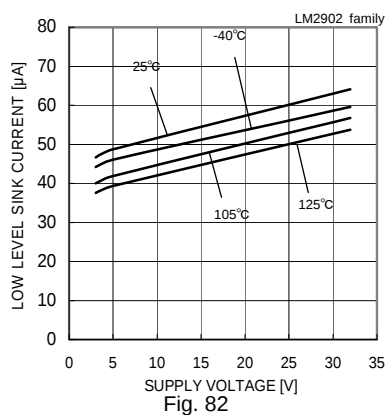
Fig. 82 Low Level Sink Current – Supply Voltage ( V_{OUT}=0.2[V] )
