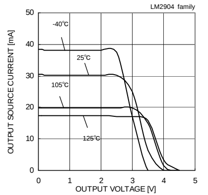
Fig. 54 Output Source Current – Output Voltage ( V_{CC}=5[V] )
