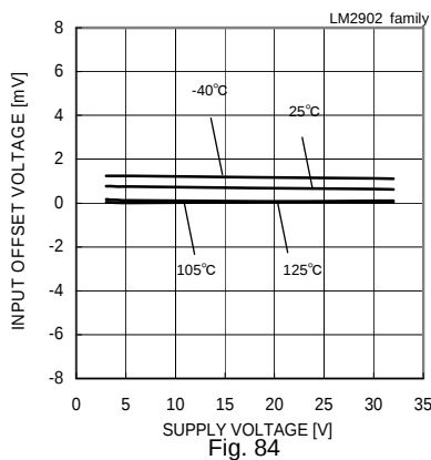
Fig. 84 Input Offset Voltage – Supply Voltage ( V_{icm}=0[V] , V_{OUT}=1.4[V] )
