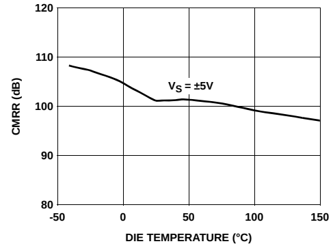
FIGURE 36. CMRR vs TEMPERATURE
