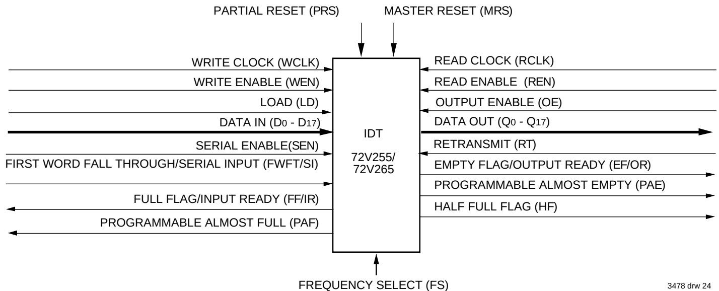
Figure 21. Block Diagram of Single 8,192x18/16,384x18 Synchronous FIFO
