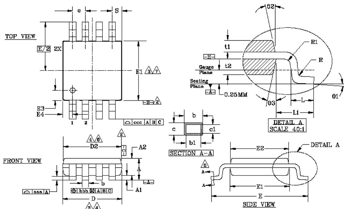
Figure 8. MSOP-8 Package
