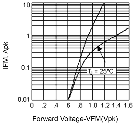
Figure 2 - Forward Characteristics
