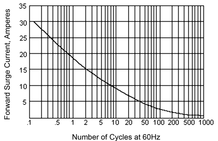
Figure 5 - Peak Forward Surge Current
