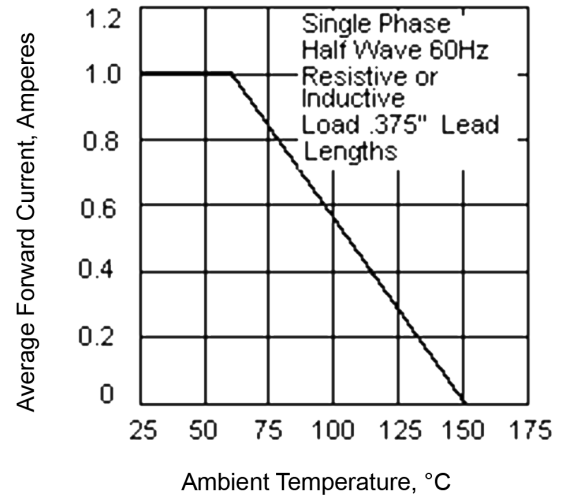
Figure 3 - Forward Current Derating Curve
