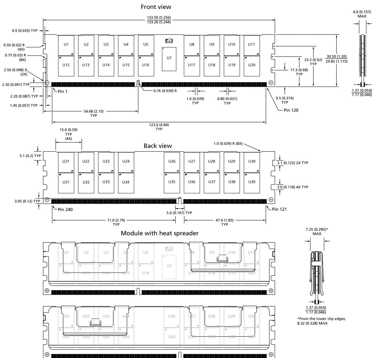
Figure 3: 240-Pin DDR3 RDIMM
