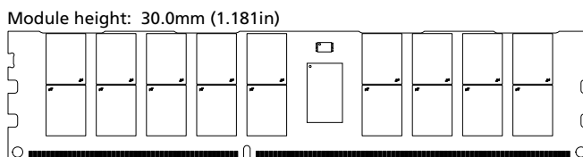
Figure 1: 240-Pin RDIMM (MO-269 R/C H)
