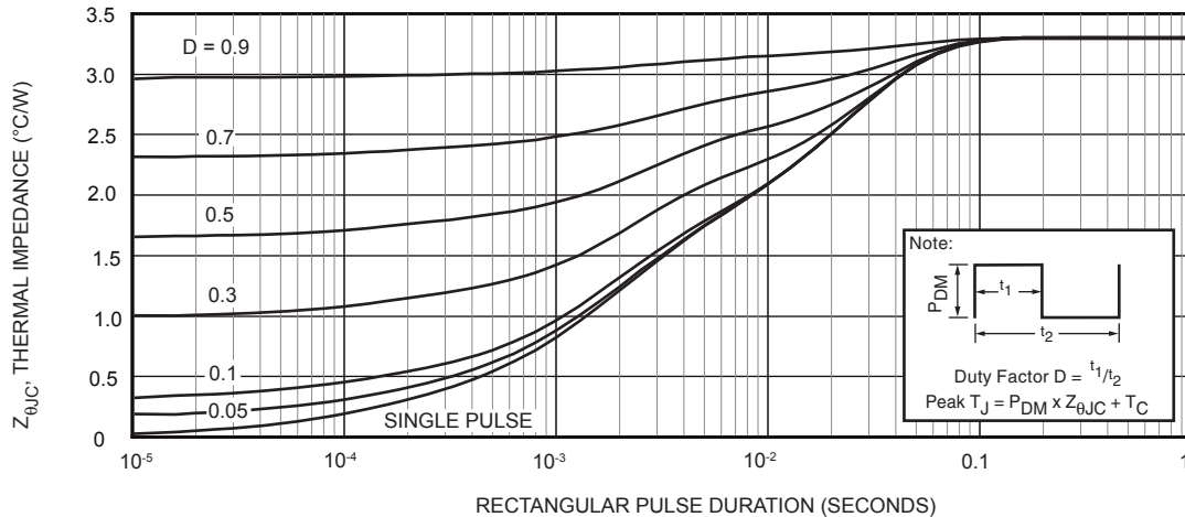
Figure 12, 15F50KF Maximum Effective Transient Thermal Impedance, Junction-To-Case vs Pulse Duration
