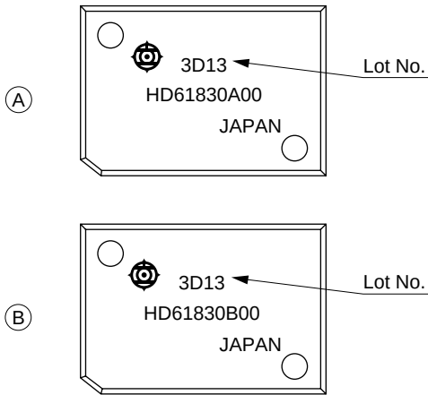
Package Marking
