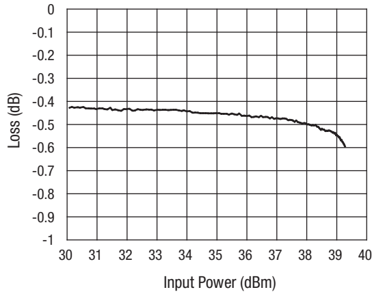
Typical Loss vs. Input Power 2500 MHz V_{CTL} = 3.3 V
