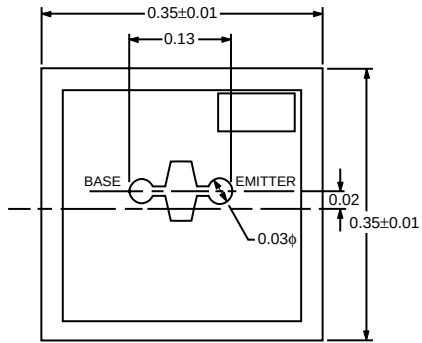
PACKAGE OUTLINE 18
