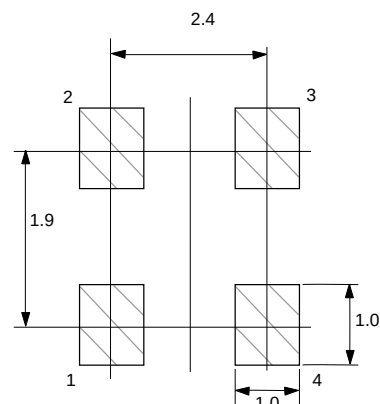
PACKAGE OUTLINE 39R RECOMMENDED P.C.B. LAYOUT
