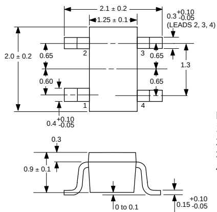
PACKAGE OUTLINE 19
