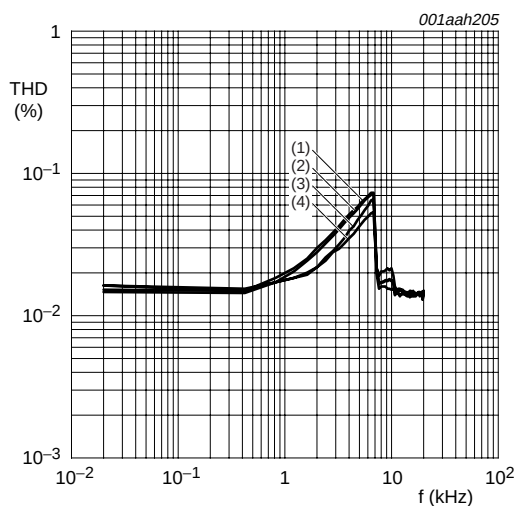
Fig 17. Total harmonic distortion as a function of frequency, BTL application with 2 Ω load
