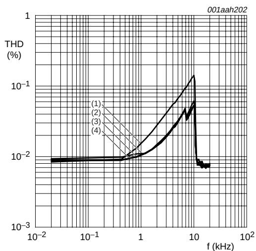
Fig 14. Total harmonic distortion as a function of frequency, SE application with 2 \Omega load
