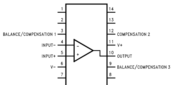
Dual-In-Line Package
