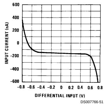
Input Current
