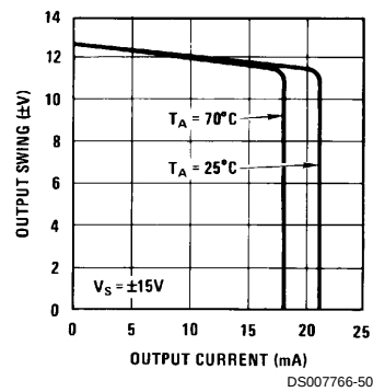
Current Limiting
