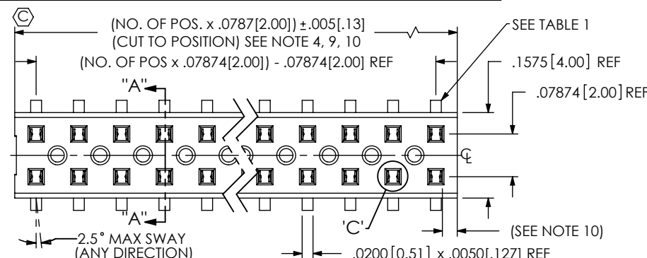
FIG 6 -BE OPTION (SAME AS FIG 1 EXCEPT INSULATOR)
