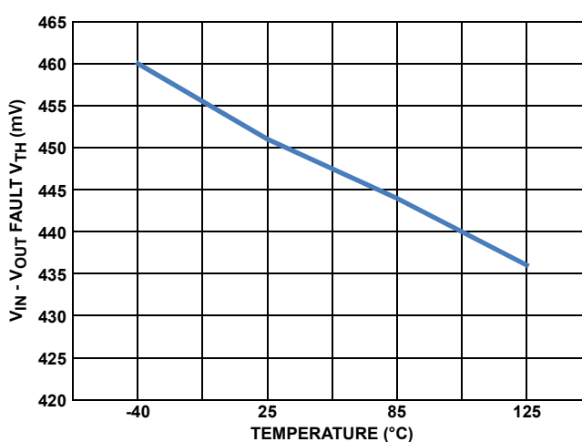
FIGURE 20. V_{\text{IN}} TO V_{\text{OUT}} FORWARD FAULT VOLTAGE
