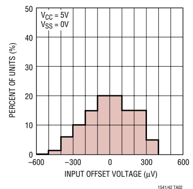
Op Amp V_{OS} Distribution, V_{CM} = 2.5V , SO-8 Package Total of 839 Units
