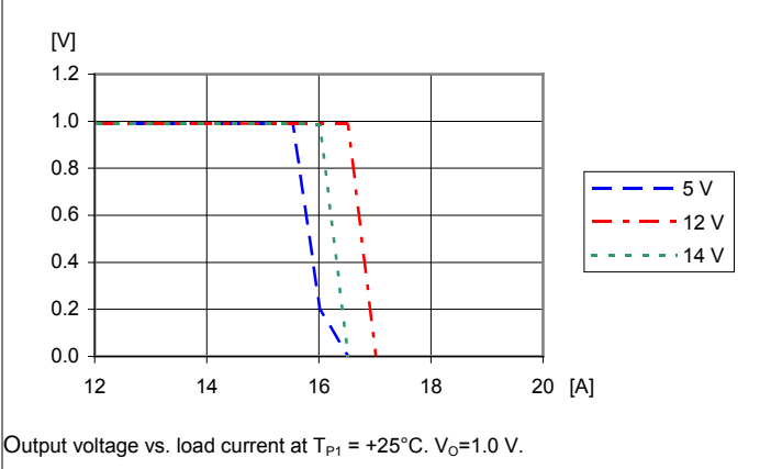
Current Limit Characteristics, V_O=1.0\text{ V}
