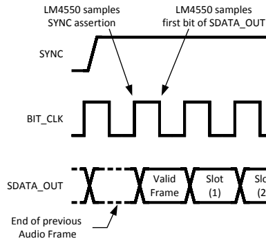
Figure 21. Start of AC Link Output Frame
