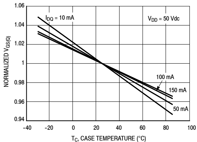
Figure 3. Normalized V_{GS(Q)} and Quiescent Current versus Case Temperature
