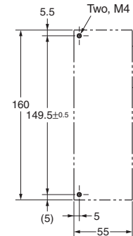
Mounting hole dimensions
