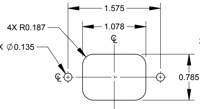
RECOMMENDED FRONT MOUNTING CUT-OUT
