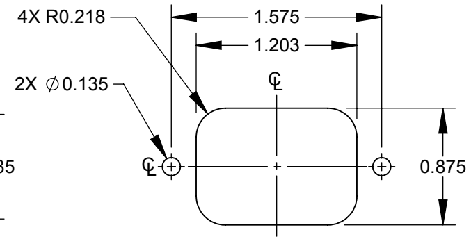
RECOMMENDED REAR MOUNTING CUT-OUT
