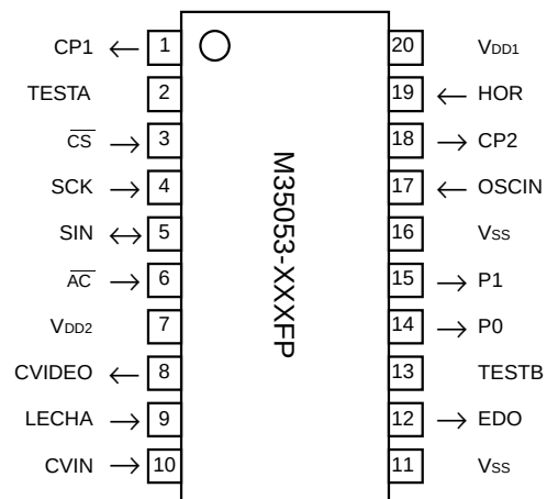
Outline 20P2Q-A
