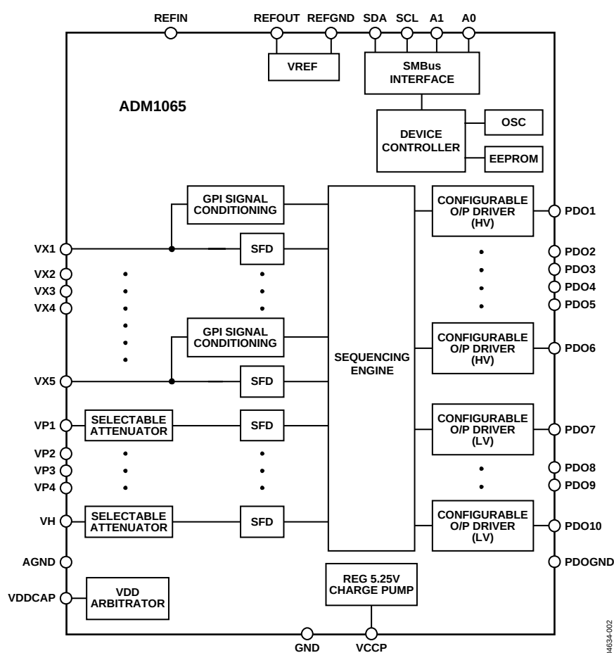
Figure 2. Detailed Block Diagram
