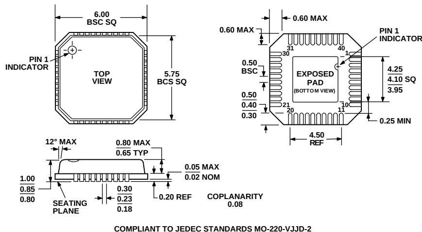
Figure 38. 40-Lead Lead Frame Chip Scale Package [LFCSP] (CP-40) Dimensions shown in millimeters
