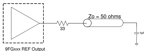
Figure 5. REF Output Test Load
