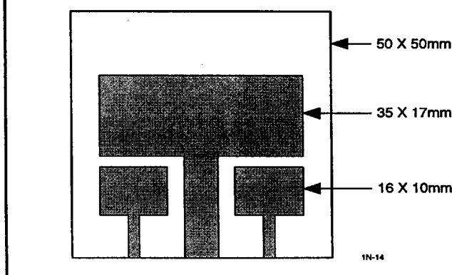
FIGURE 2. SUBSTRATE LAYOUT FOR SOT-223
