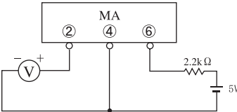
Fig1. Measurement Circuit
