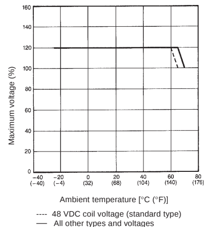
Ambient temperature vs. maximum voltage
