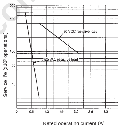
Electrical service life
