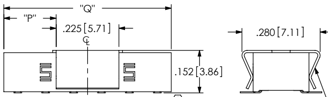
FIGURE 5 (-P: PICK & PLACE PAD)
