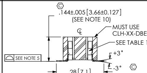
FIG 4 (-BE: BOTTOM MOUNT ENTRY)
