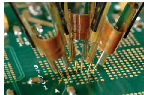
The Probe Tip Modules contain the active amplifier circuitry. Different modules have different electrical and physical interconnect characteristics, allowing the user to select the module appropriate for the application.
