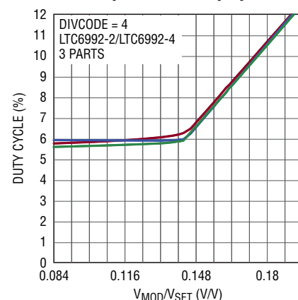
Linearity Near 5% Duty Cycle
