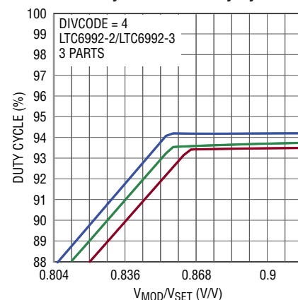
Linearity Near 95% Duty Cycle
