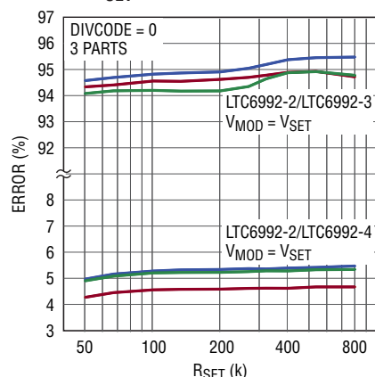
N_{DIV} = 1 Duty Cycle Clamps vs R_{SET}
