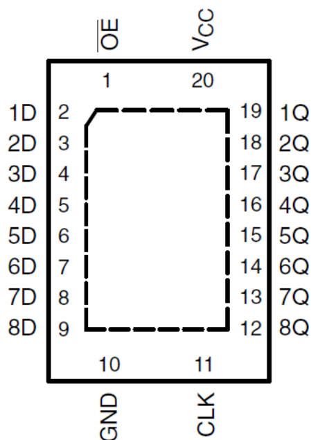
Figure 5-2. RGY Package (Top View)
