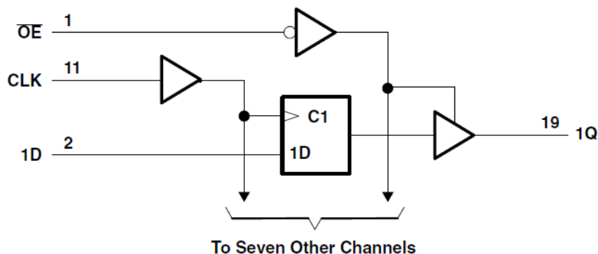
Logic Diagram (Positive Logic)
