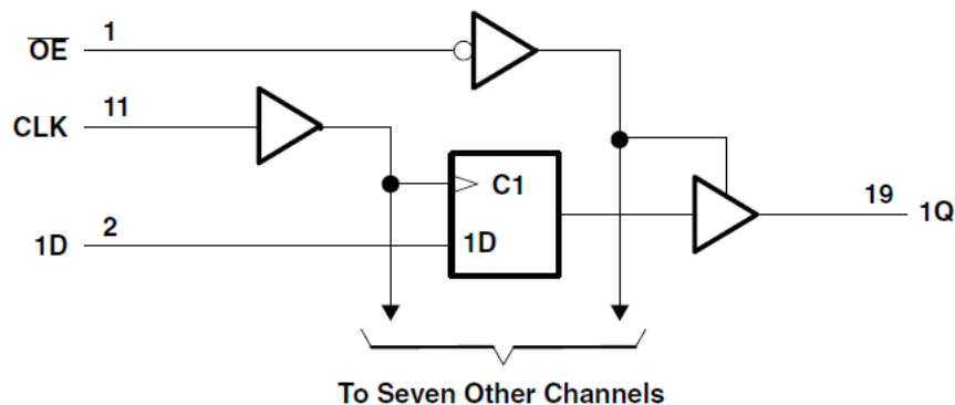
Figure 8-1. Logic Diagram (Positive Logic)
