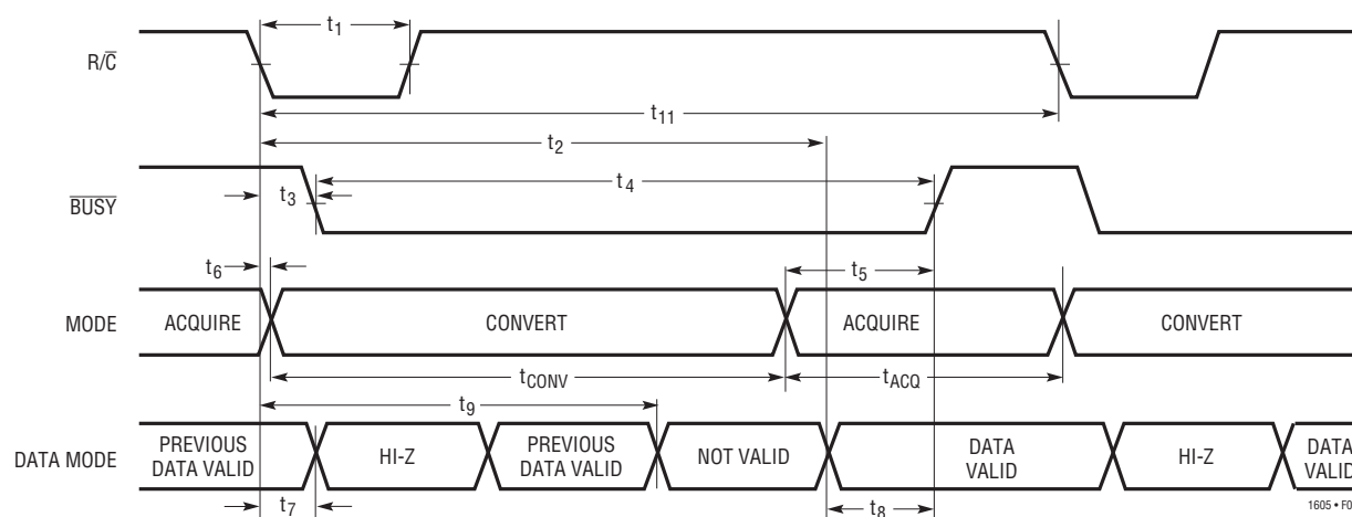
Figure 8. Conversion Timing with Outputs Enabled After Conversion ( \overline{\text{CS}} Tied Low)
