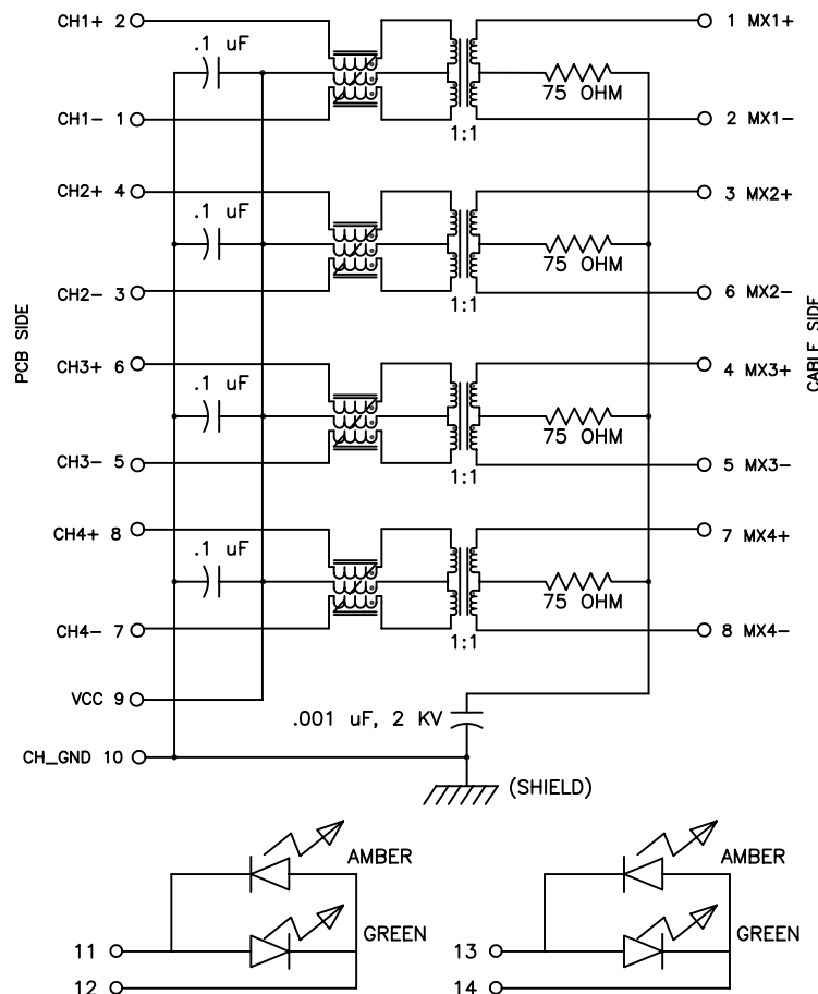
SCHEMATIC
