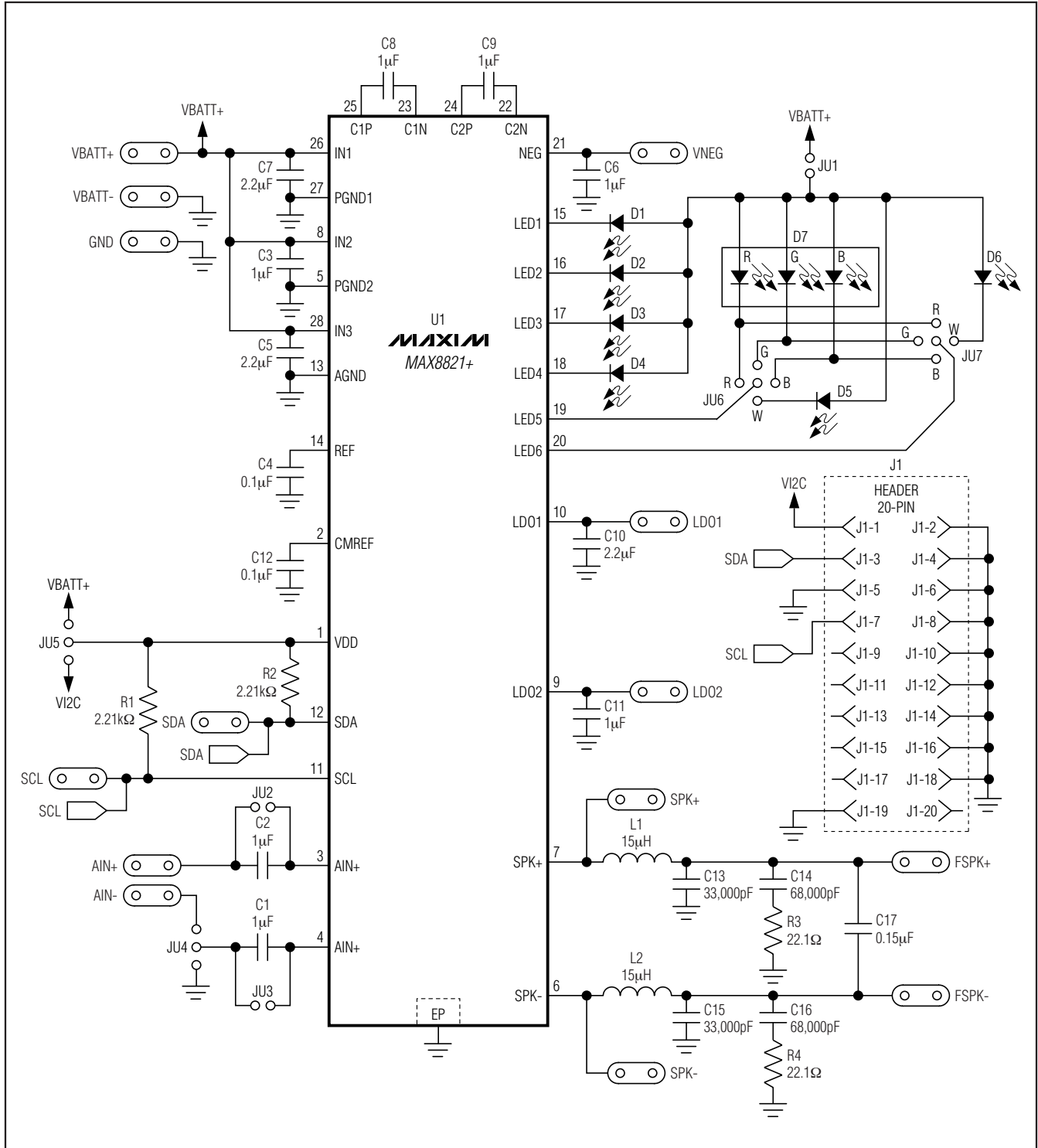
Figure 5. MAX8821 EV Kit Schematic
