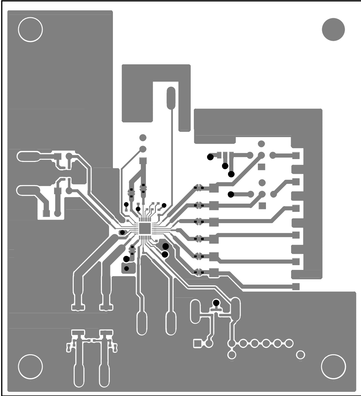
Figure 7. MAX8821 EV Kit PCB Layout—Component Side
