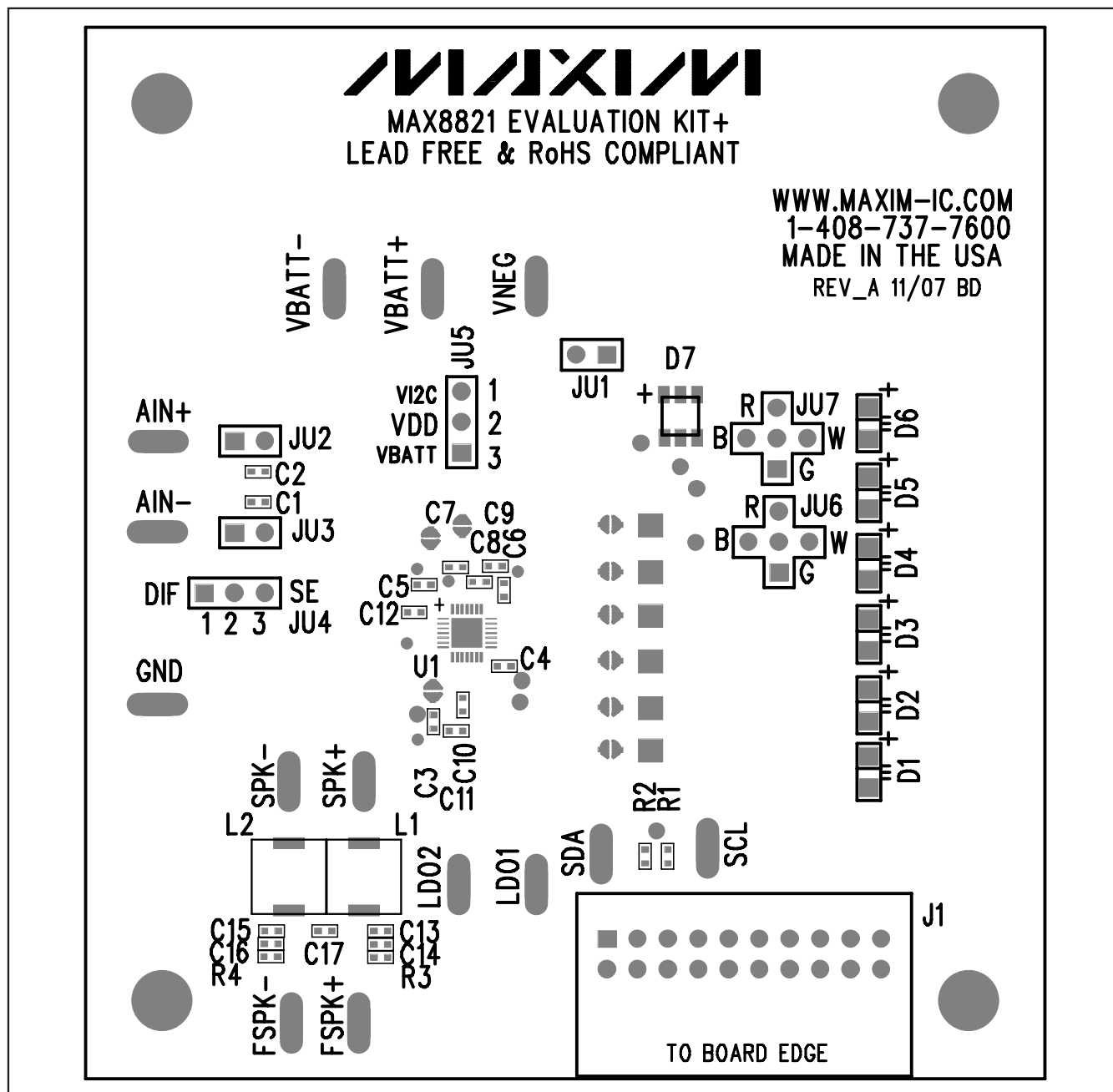
Figure 6. MAX8821 EV Kit Component Placement Guide—Component Side
