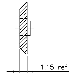
SECTION Z-Z
