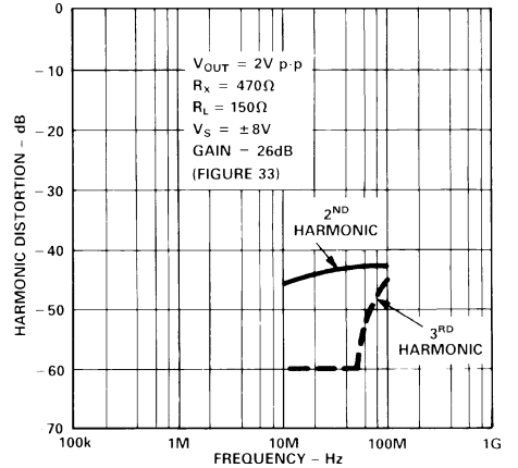
Figure 9. Harmonic Distortion vs. Frequency - High Gain
