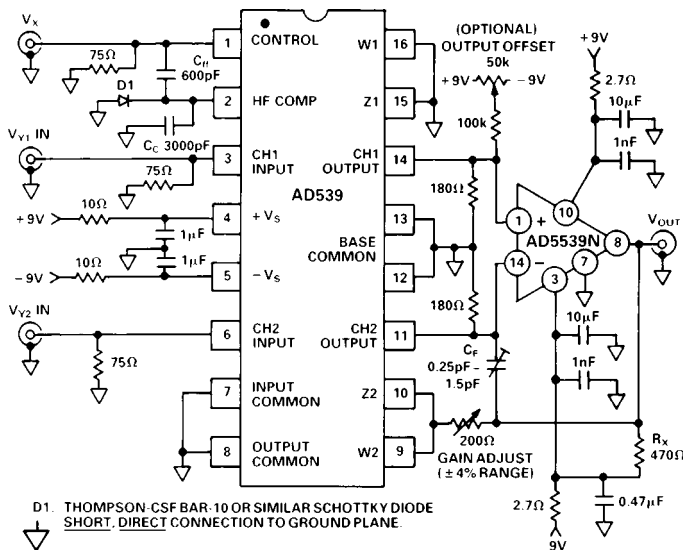
Figure 44. A Wide Bandwidth Voltage-Controlled Amplifier
