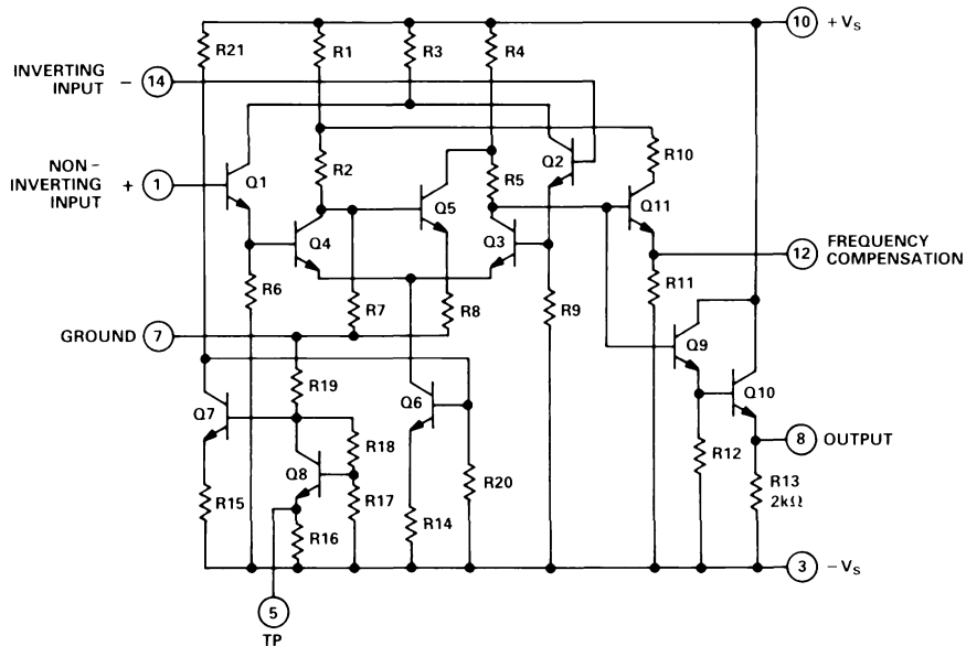
Figure 12. AD5539 Circuit
