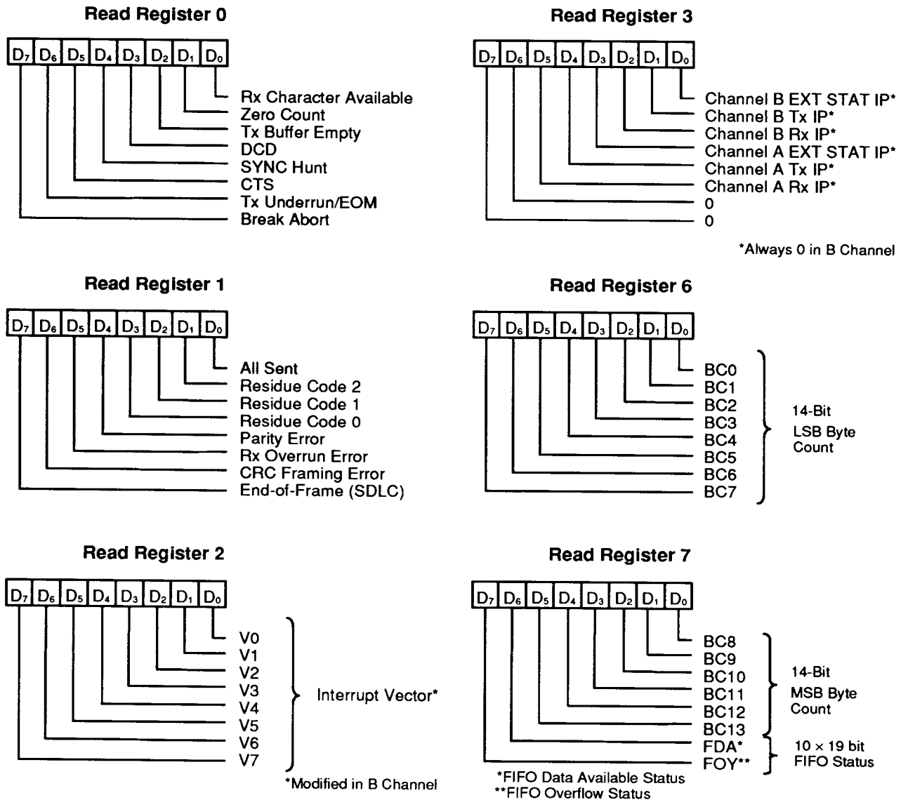
Figure 8. Read Register Bit Functions
