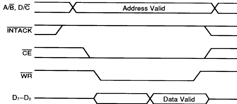
Figure 10. Read Cycle Timing
