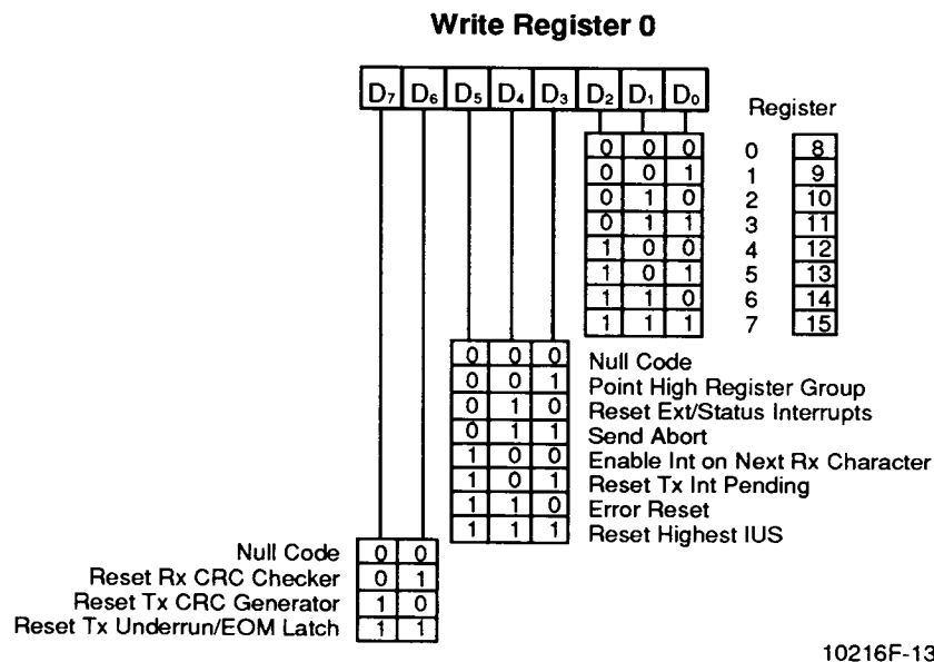
Figure 9. Write Register Bit Functions
