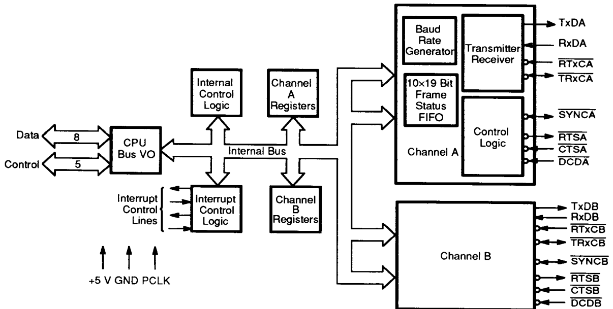
Figure 1. Block Diagram of ESCC Architecture
