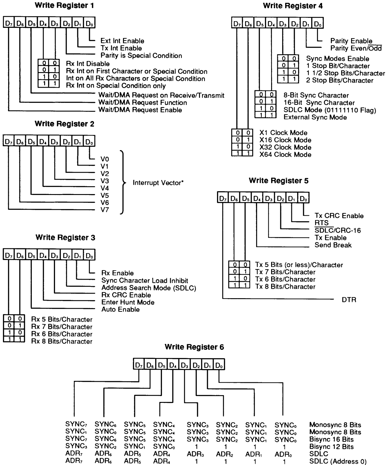
Figure 9. Write Register Bit Functions (continued)
