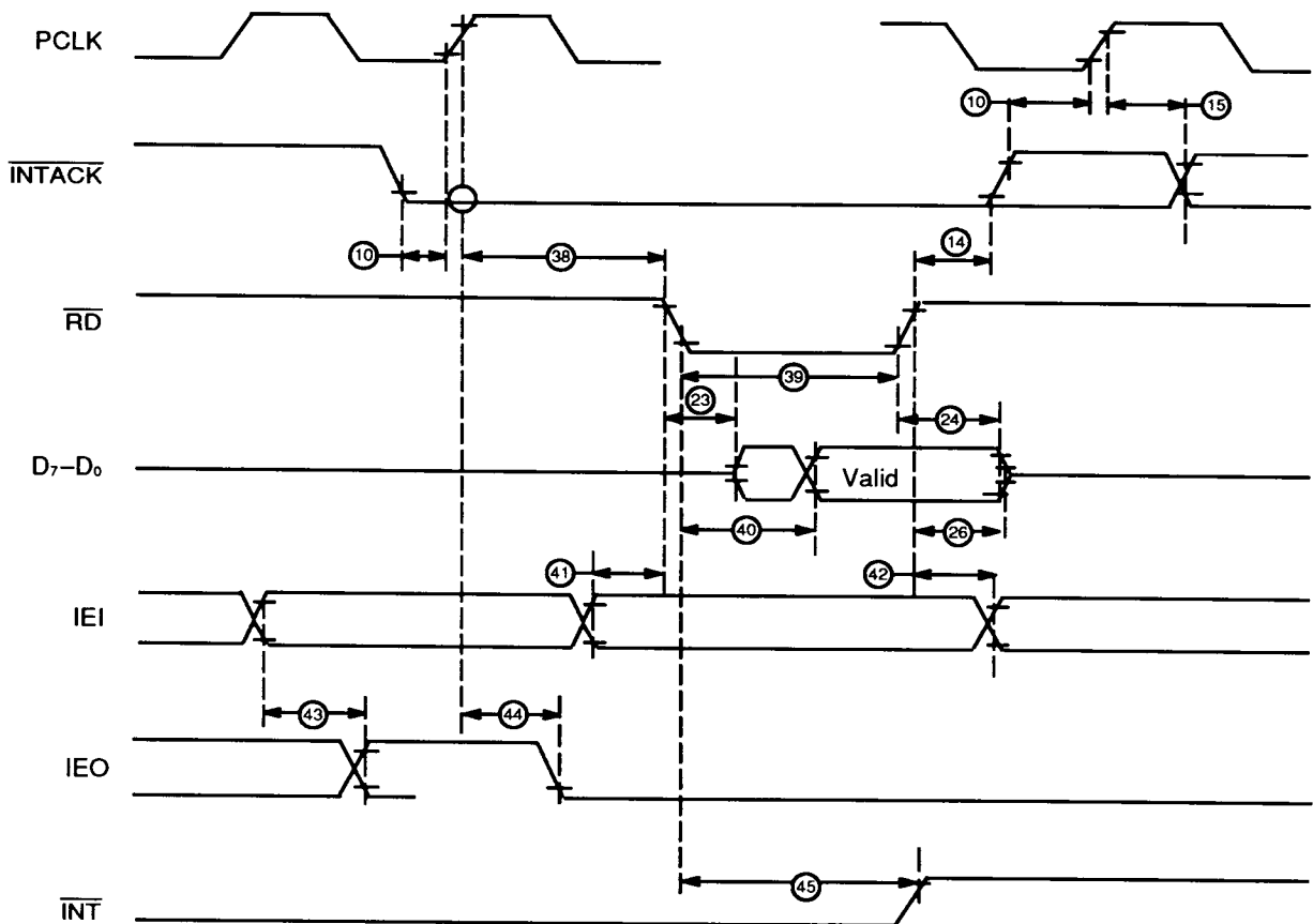
Figure 24. Interrupt Acknowledge Timing
