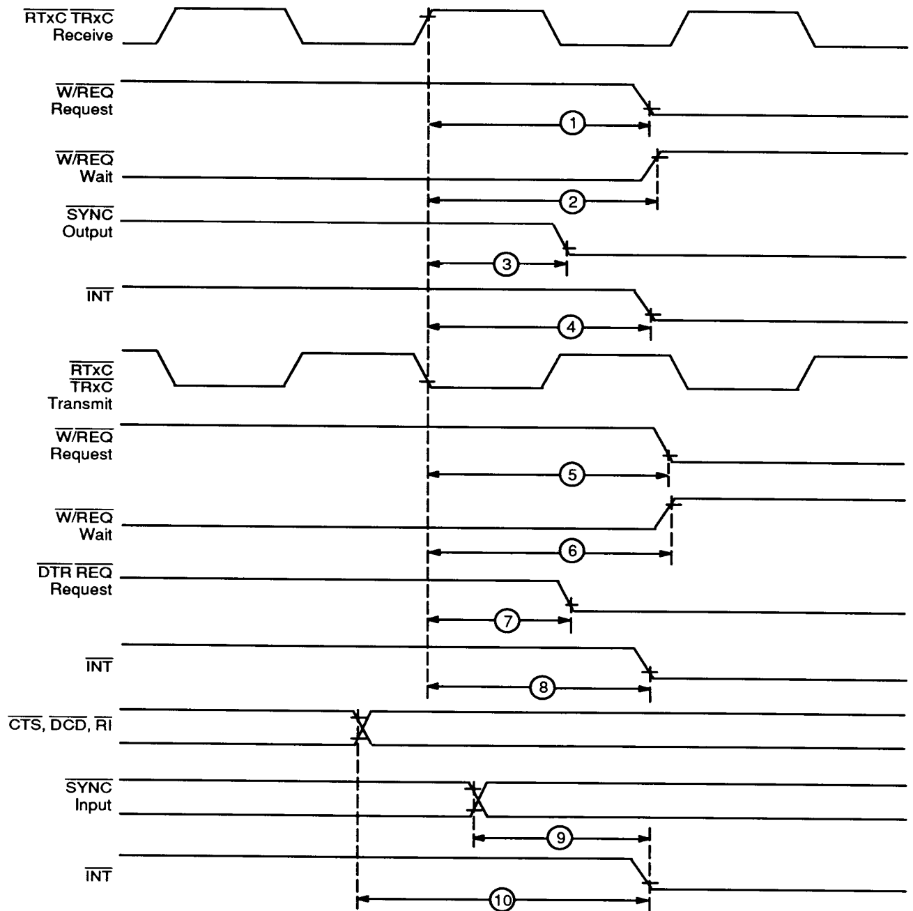
Figure 20. System Timing
