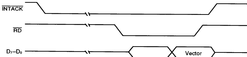
Figure 12. Interrupt Acknowledge Cycle Timing
