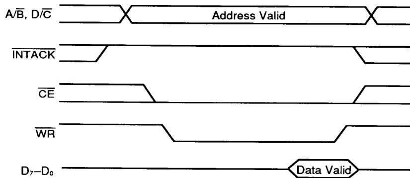
Figure 11. Write Cycle Timing
