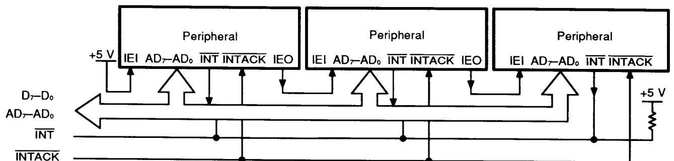
Figure 7. Z-Bus Interrupt Schedule
