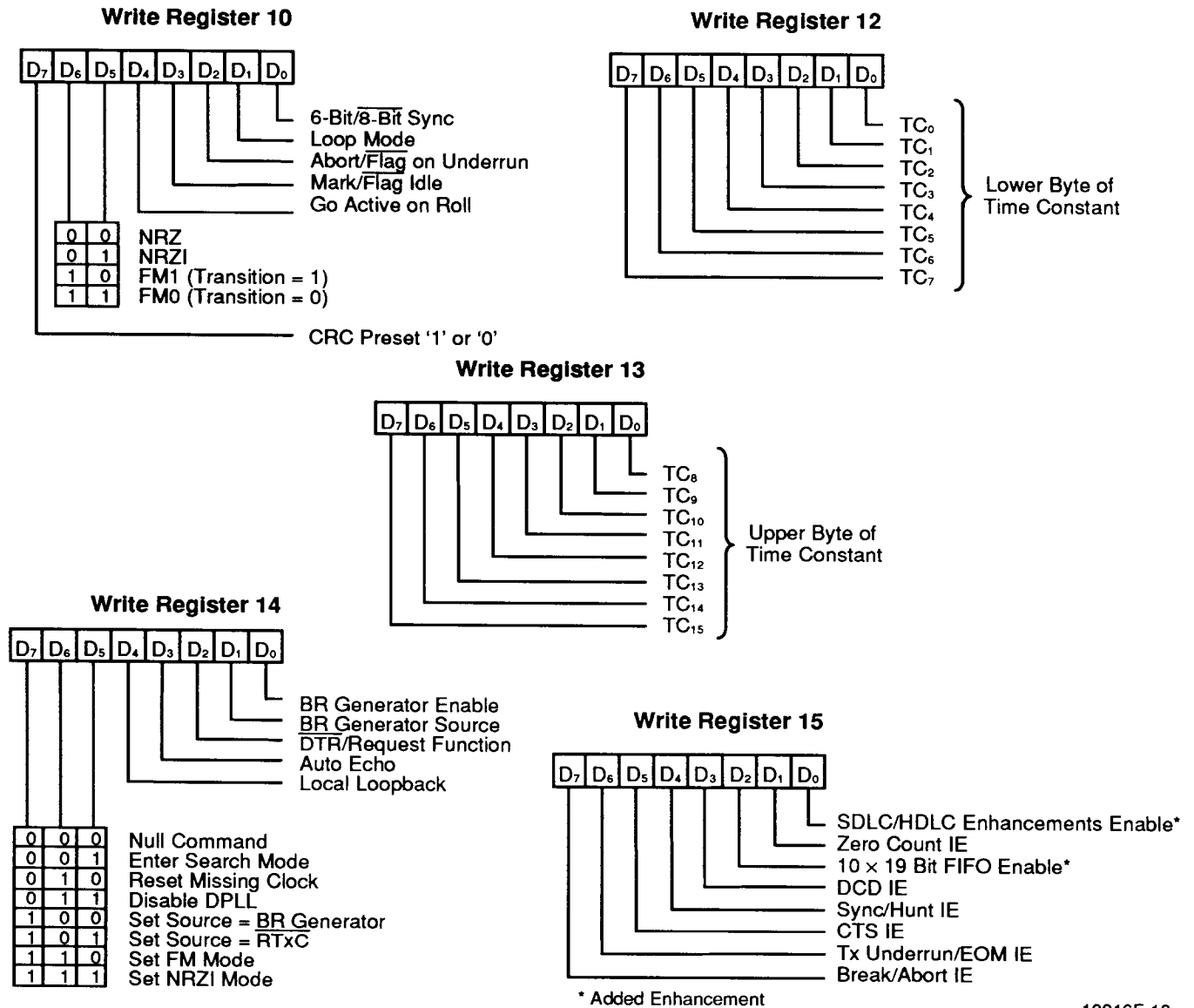
Figure 9. Write Register Bit Functions (continued)
