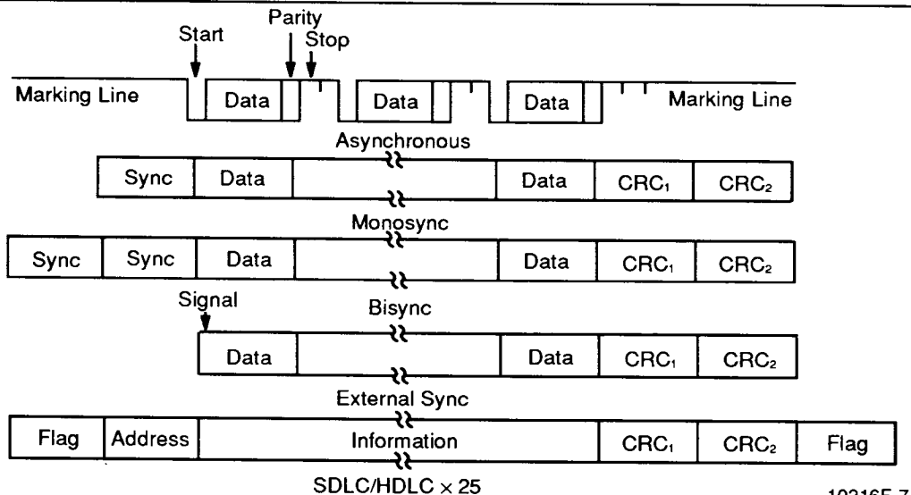
Figure 3. SCC Protocols
