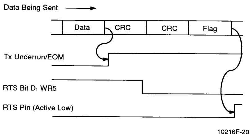
Figure 16. Auto \overline{\text{RTS}} Reset Mode
