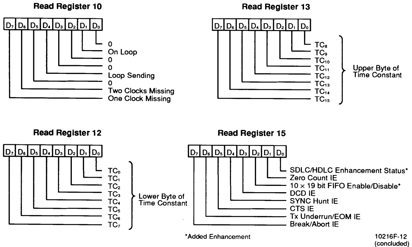
Figure 8. Read Register Bit Functions (continued)
