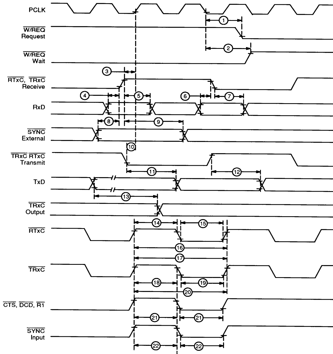
Figure 19. General Timing
