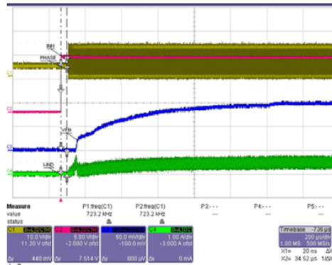
Figure 24. Soft-start
