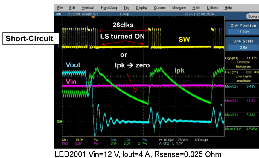
Figure 18. Constant current protection triggering hiccup mode
