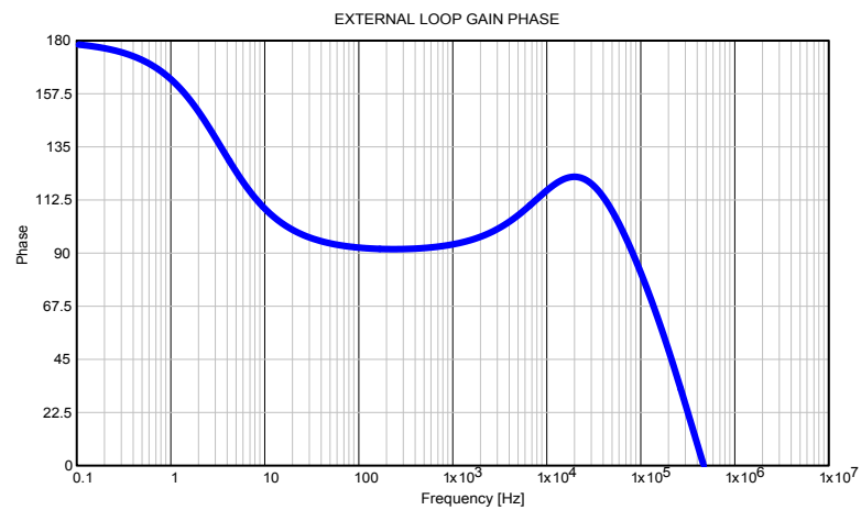
Figure 10. Phase plot
