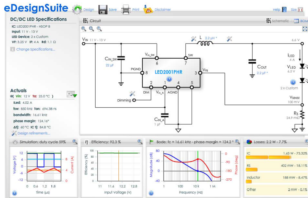
Figure 14. eDesignSuite software
