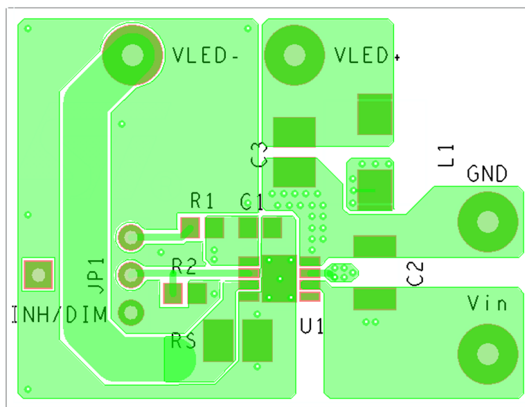
Figure 16. Layout example
