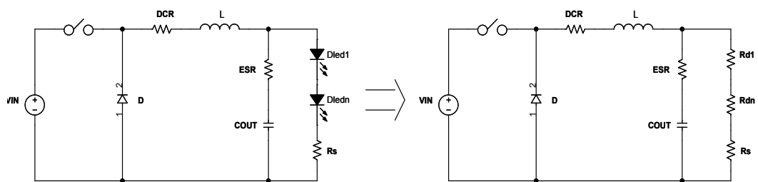
Figure 15. Equivalent circuit
