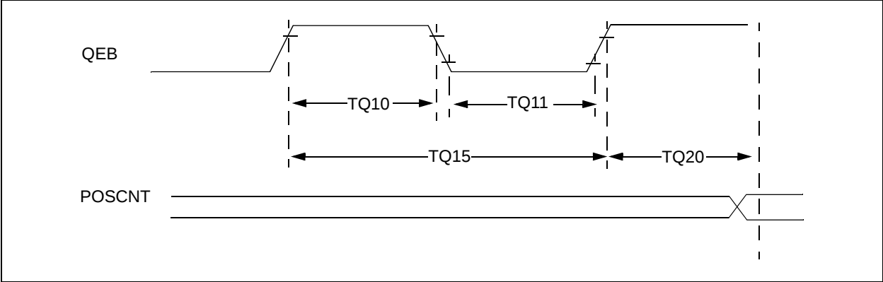
FIGURE 24-8: TIMERQ (QE1 MODULE) EXTERNAL CLOCK TIMING CHARACTERISTICS
