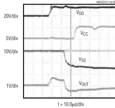
BIPOLAR STARTUP RESPONSE, C_{LOAD} = 250pF
