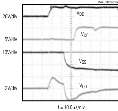
BIPOLAR STARTUP RESPONSE, C_{LOAD} = 10pF
