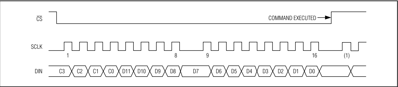
Figure 2. Serial-Interface Signals
